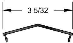
30° OUTSIDE MULL
