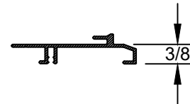
CLAD BRICKMOULD SUBSILL EXTRUSION
