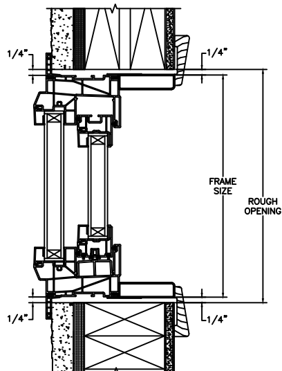
HEAD JAMB & SILL 2 X 4 FRAME WITH STUCCO 1" OR 2" FLANGE OPTION
