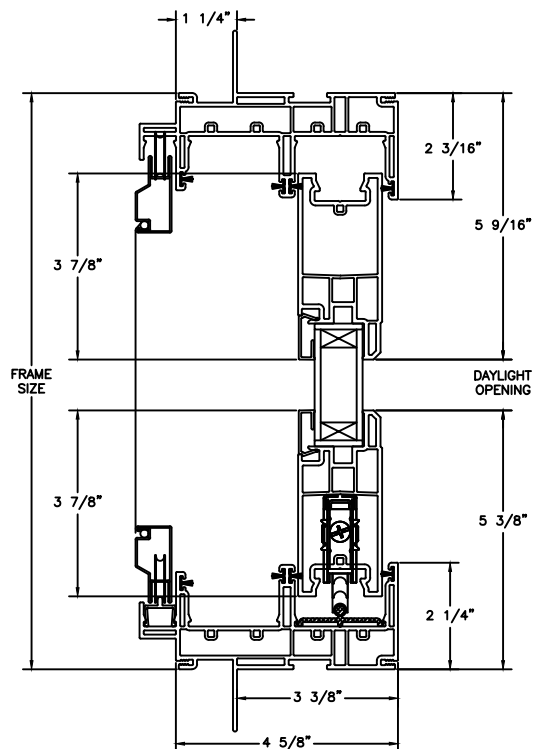
OPERATING HEAD JAMB & SILL
