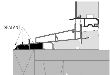
FIG. 18: IN-SWING SILL
